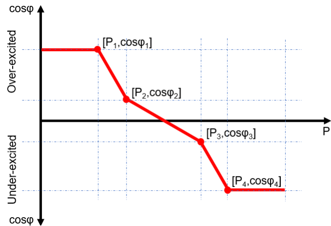
Abb. 191. Cos-phi(P)-Kurve
