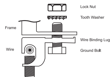
Figure 7: Installation Methods
